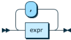
Figure 12.8 argsList
