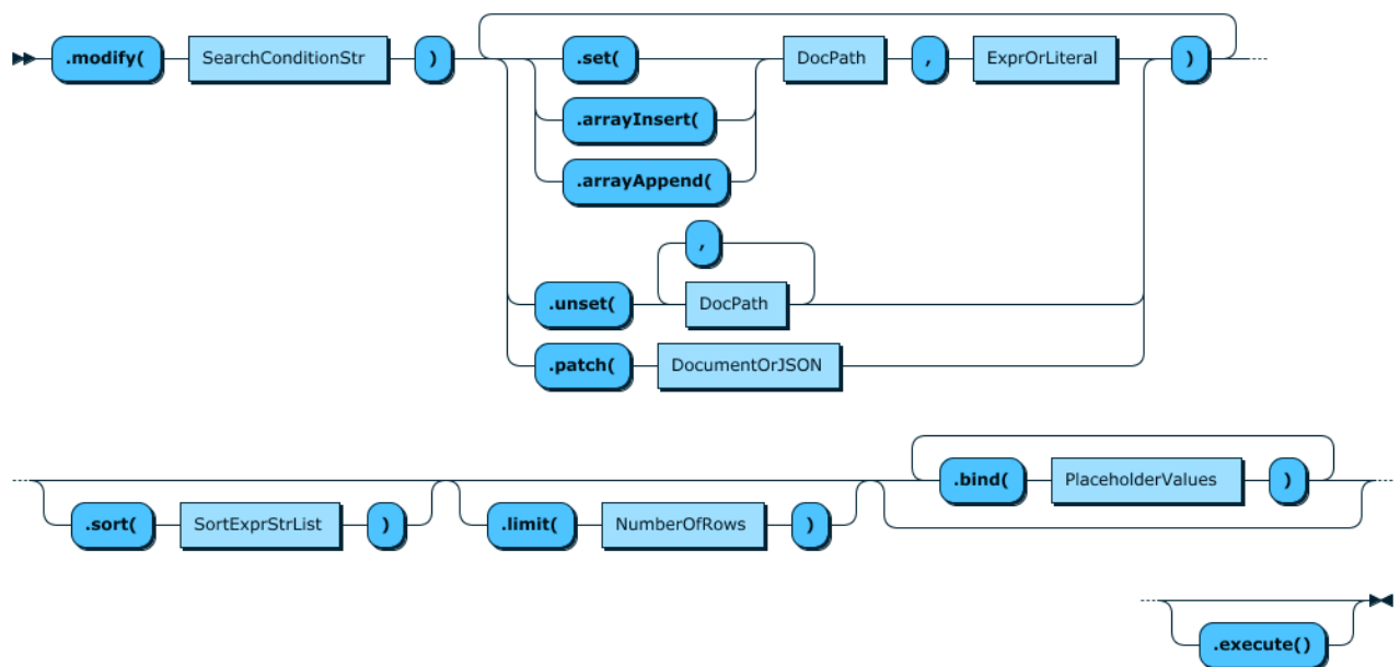
Figure 11.10 CollectionModifyFunction
